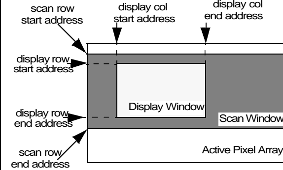
Figure 13. Windowing
